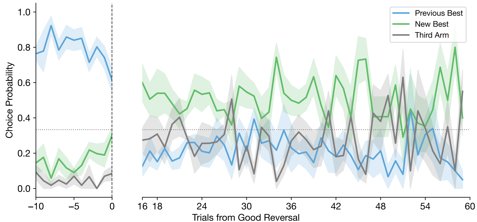
Good Reversal-Aligned Choices (mean \pm se across subjects | n=5 subjects, n=45 reversals) (Skipping first 15 trials post-reversal)
